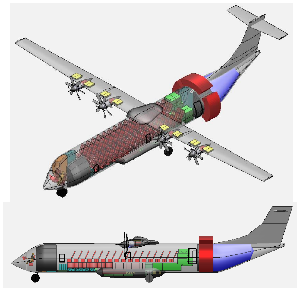
Figure 8: Conceptual fuel cell fully electric 80-pax regional aircraft
