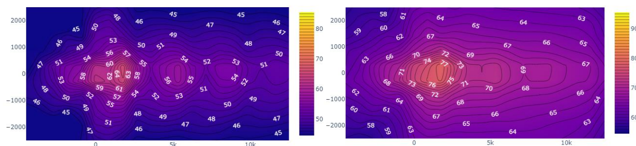
Figure 6 – Left: Maximum Sound Pressure Levels [dB] for C7A-HARW aircraft on the ground through the entire departure procedure. Right: Sound Exposure Levels on the ground for the entire departure procedure for C7A-HARW aircraft. Source: UNIFIER19 D3.3 (UNIFIER19, September 2022).
